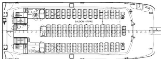
MAIN DECK
